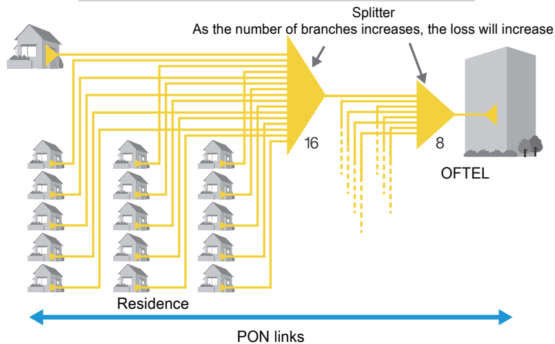
Measuring a residential PON network with two-level splitters
